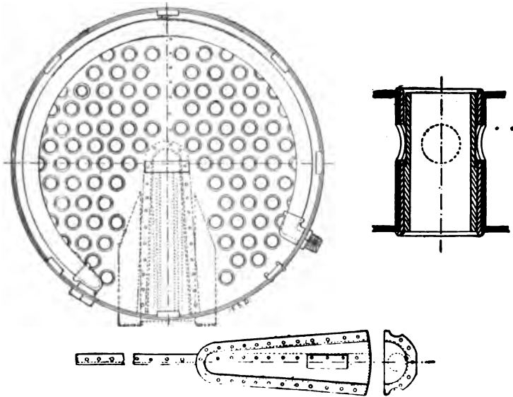
FIG. 214.—Whitney Bunsen Tube Burner of the McKay Carriage, showing section of one of the Bunsen tubes, and starting torch.
